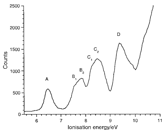
Fig. 3 He I PE spectrum of compound 1a .
